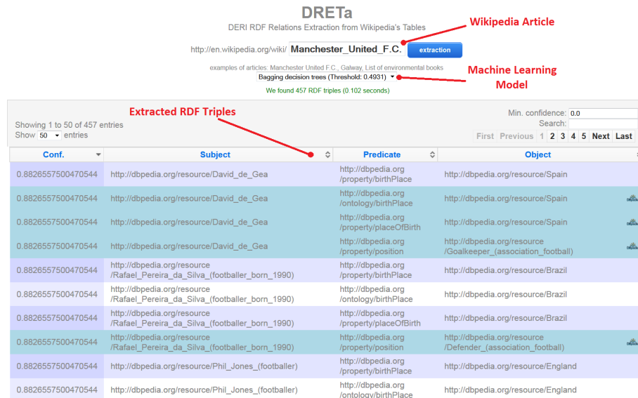
Fig. 2: DRETa demo interface showing the top triples extracted from tables in the “Manchester United F.C.” article with associated confidence scores.
